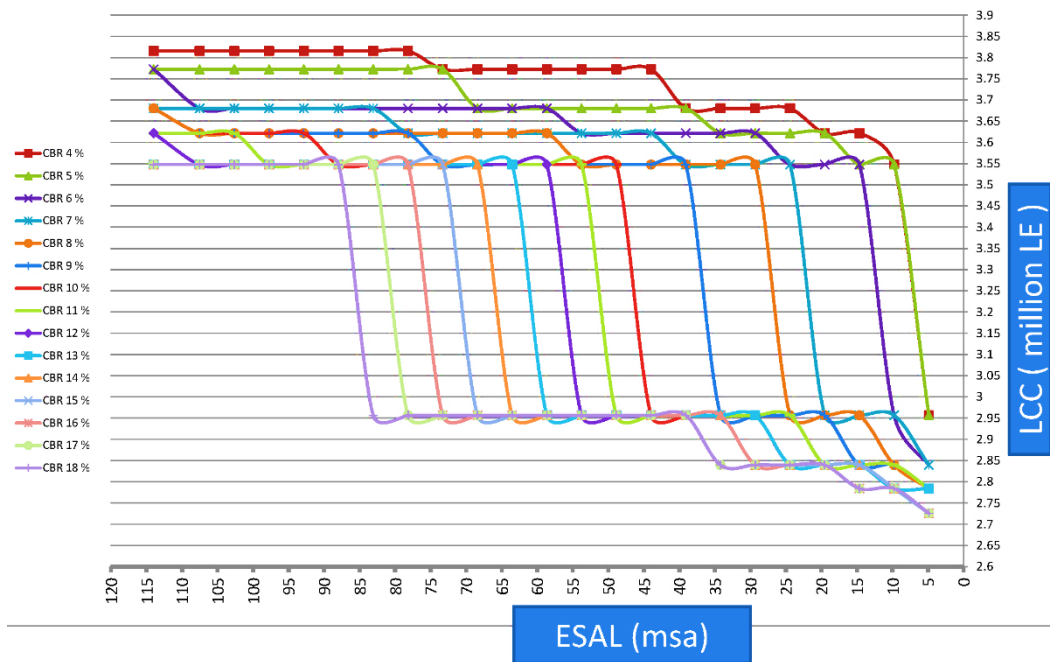
FIGURE 2. The relationship between LCC (million LE) and ESAL (msa) for flexible pavement at each value of CBR.
