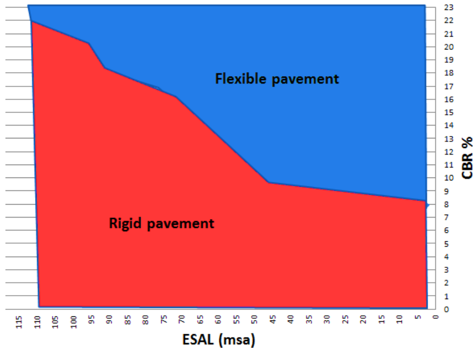
FIGURE 6. The relationship between CBR% and ESAL (msa) when considering LCC to select pavement type
