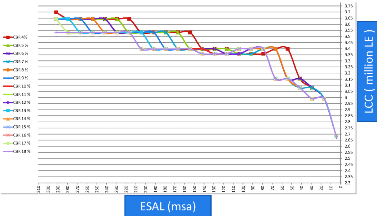
FIGURE 4. The relationship between LCC (million LE) and ESAL (msa) at each CBR value for rigid pavement.
