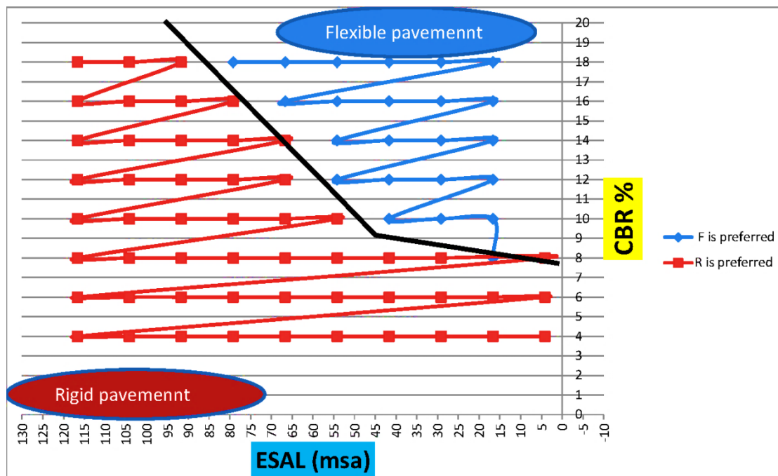
FIGURE 5. The relationship between ESAL (msa) and LCC (million LE at each value of CBR to obtain two zones of flexible and rigid pavement
